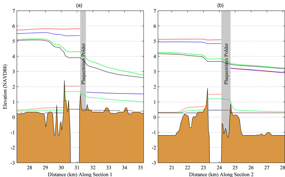
Fig. 8. (Color) Maximum Hurricane Katrina water levels along the Mississippi River: (a) Section 1; (b) Section 2; for SL16-Raised Levees scenario, red lines represent high flow ( 22,654 \text{ m}^3/\text{s} ) and blue lines represent low flow ( 5,664 \text{ m}^3/\text{s} ); for SL16-Lowered Levees scenario, green lines represent high flow and black lines represent low flow; solid lines indicate the maximum total water level and dashed lines indicate the base flow water levels
